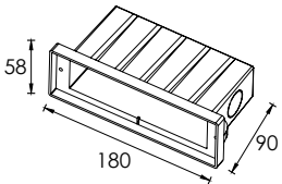
Mounting sleeve 076#
